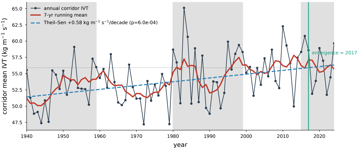
Continuous US West Coast corridor moisture-transport trajectory, 1940-2024
