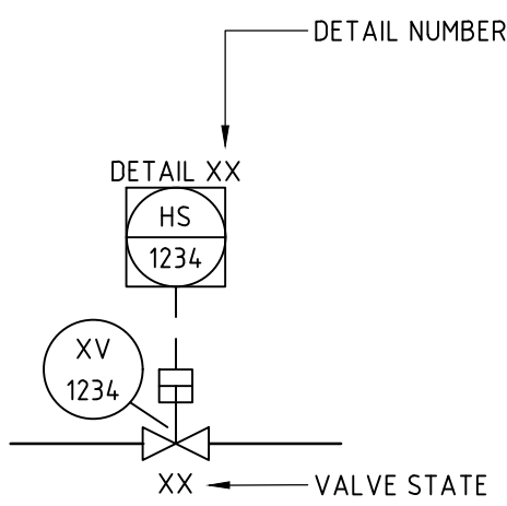
ROTARY ON / OFF VALVE
