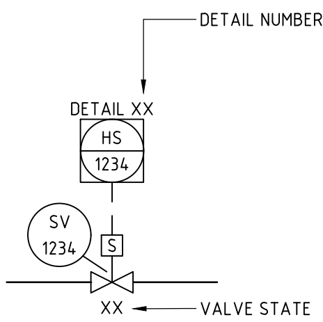
DIRECT SOLENOID VALVE
