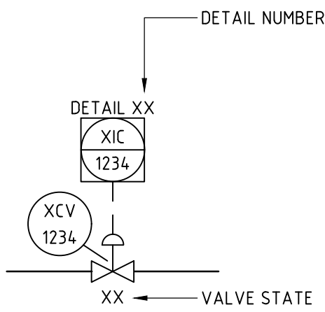
MODULATING VALVE
