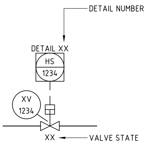
ON / OFF VALVE
