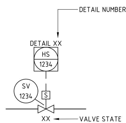
DIRECT SOLENOID VALVE
