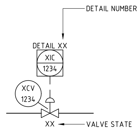
MODULATING VALVE
