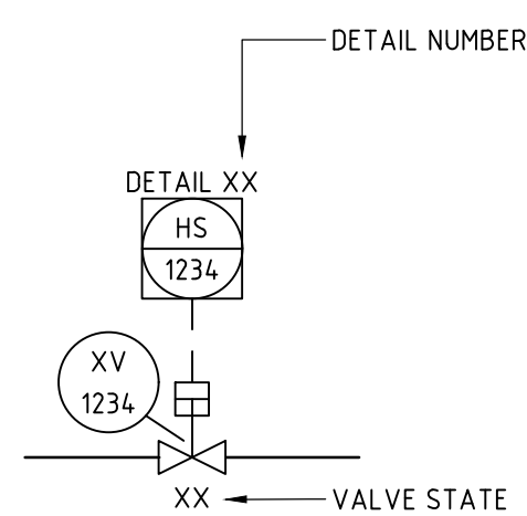
ROTARY ON / OFF VALVE
