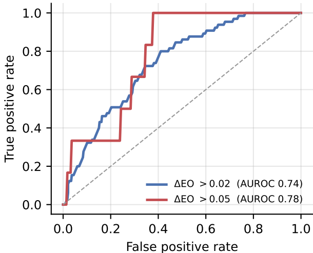
Early-warning detector (Adult)
