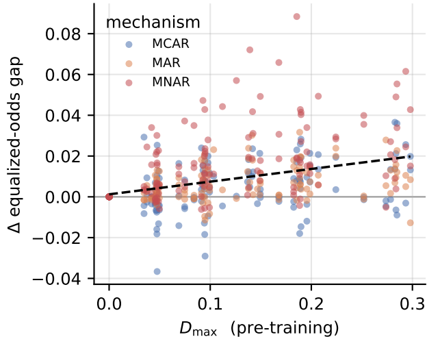
Adult: signal holds ( r = +0.40 )
