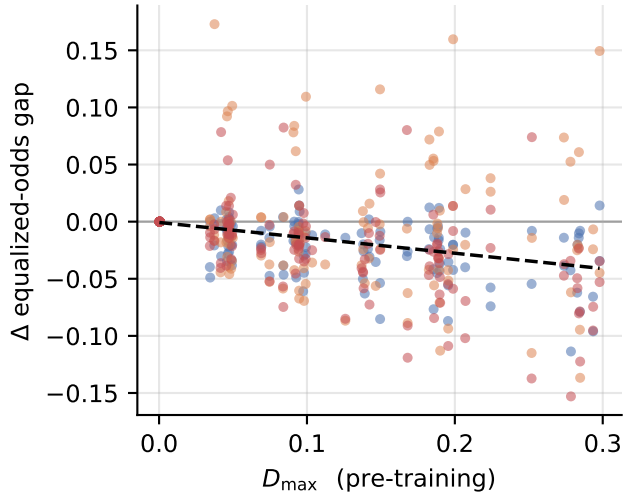
COMPAS: reverses ( r = -0.31 )
