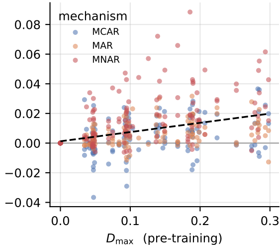
Adult: holds (n=45k) ( r = +0.40 )
