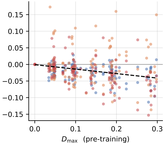
COMPAS: reverses (n=5k) ( r = -0.31 )
