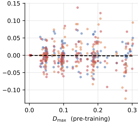
German: null (n=1k) ( r = -0.02 )
