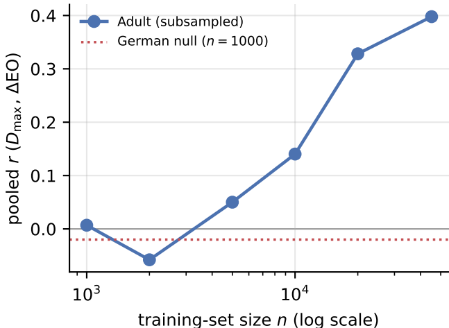
Detectability grows with sample size
