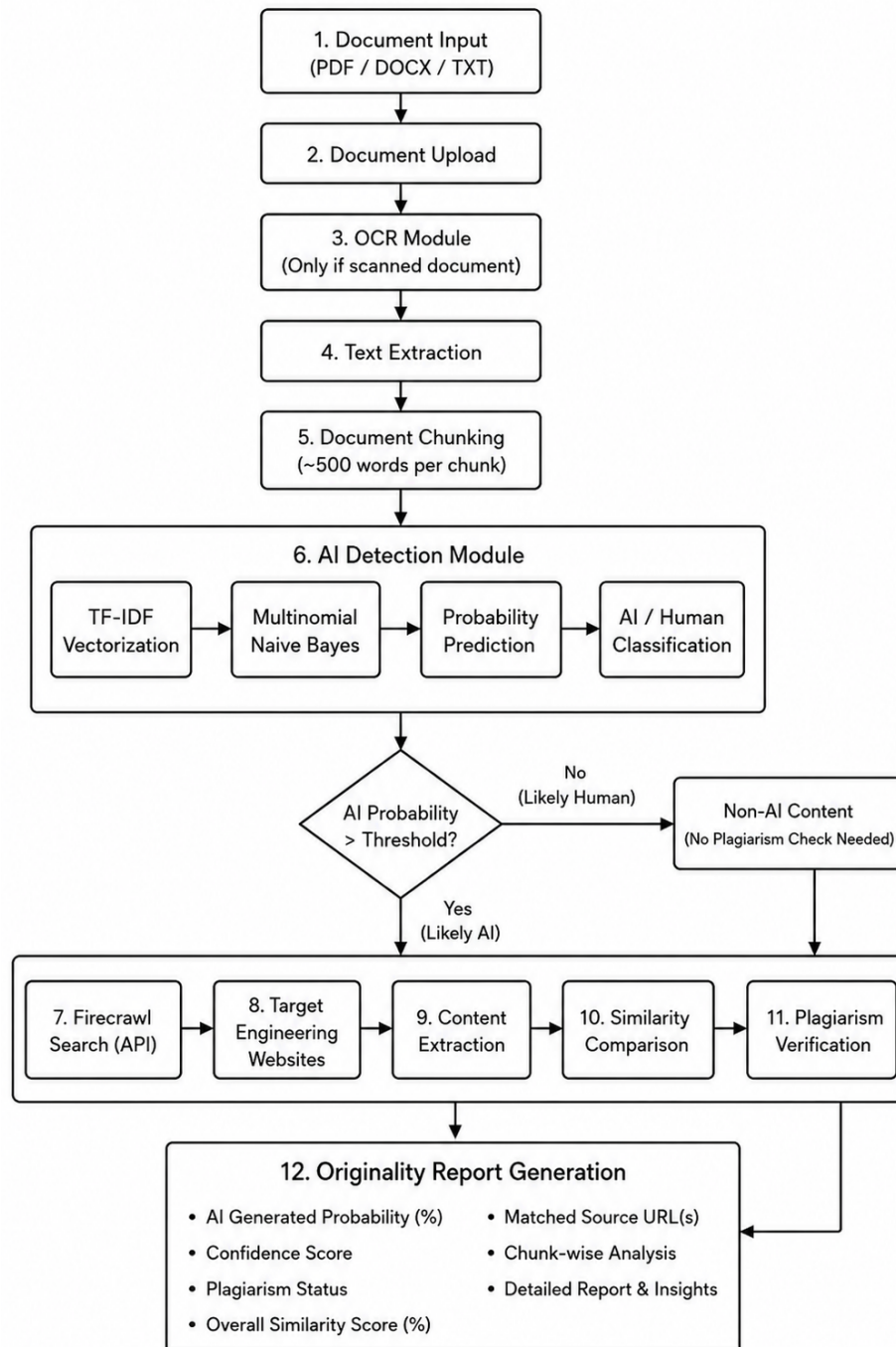
Figure 3.1: Machine Learning Model Workflow
