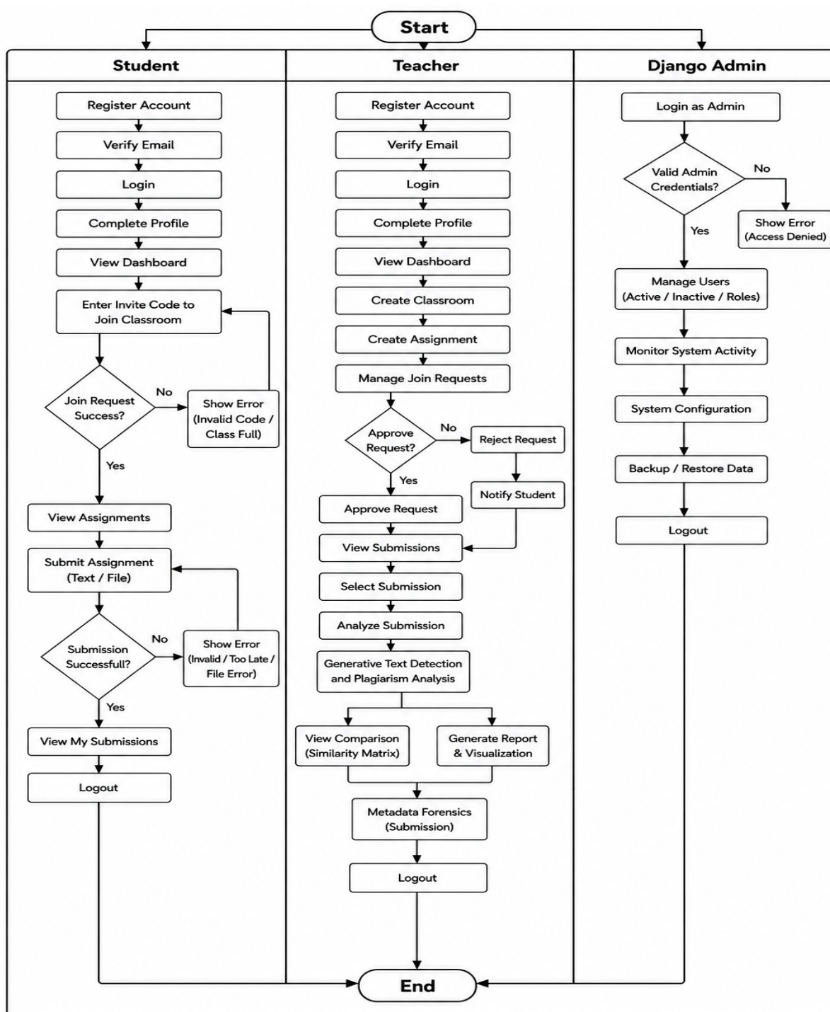
Figure 4.5: System Flowchart Showing Student, Teacher and Admin Workflows
