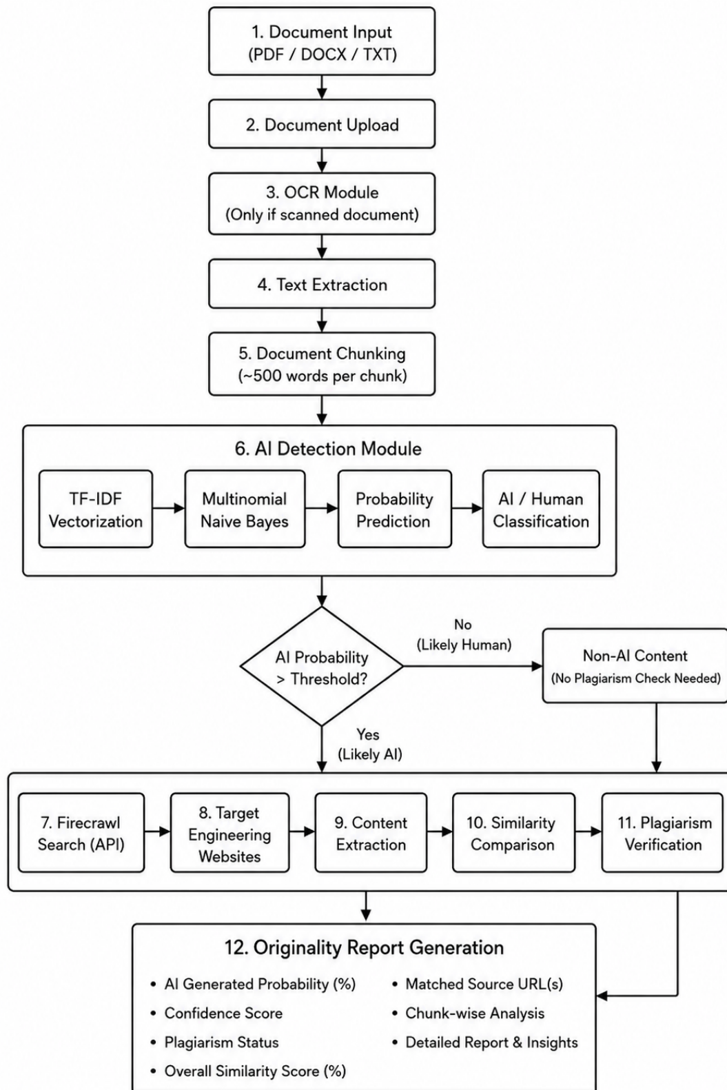
Figure 3.2: Machine Learning Model Workflow
