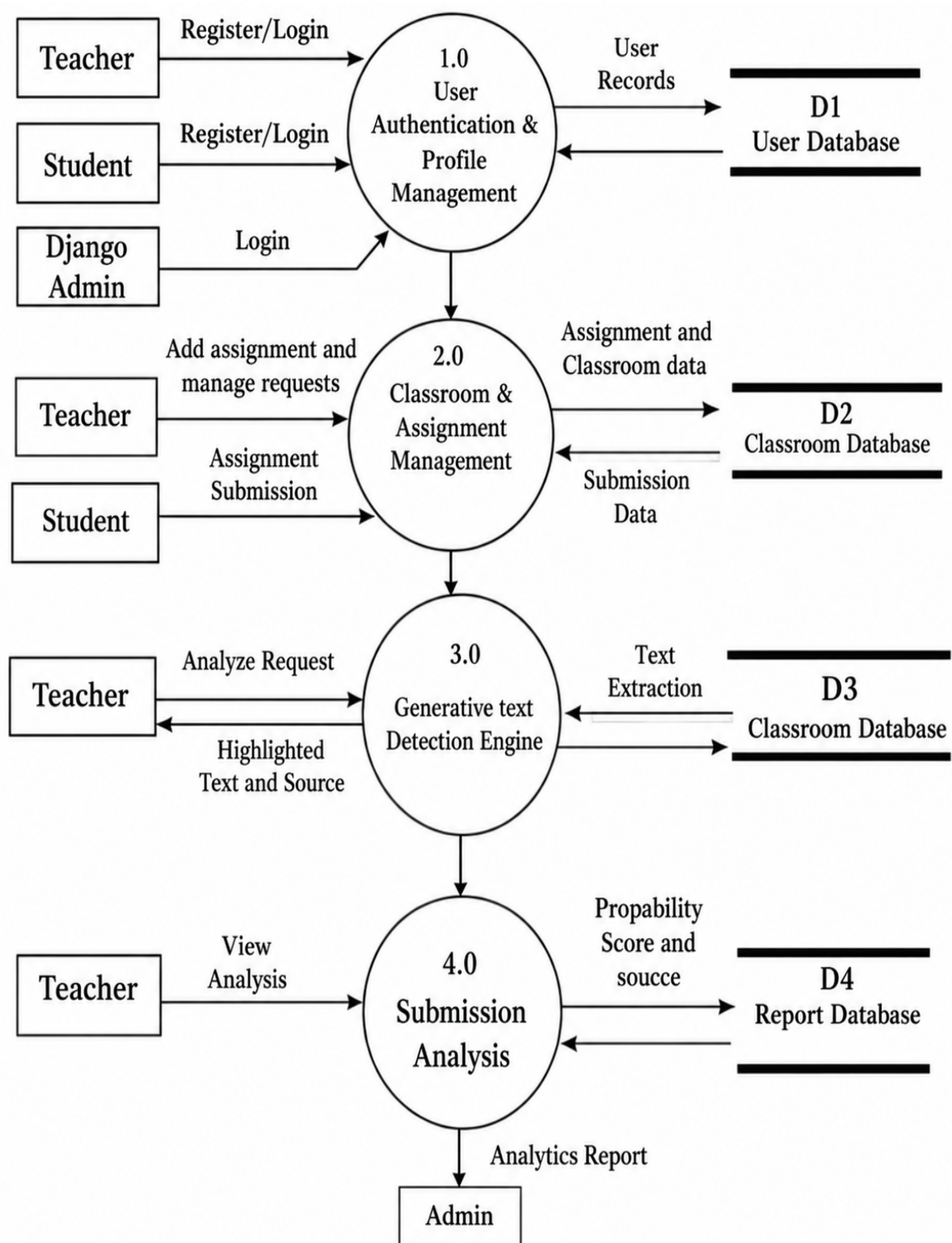
Figure 3: Level 1 Data Flow Diagram of the System
