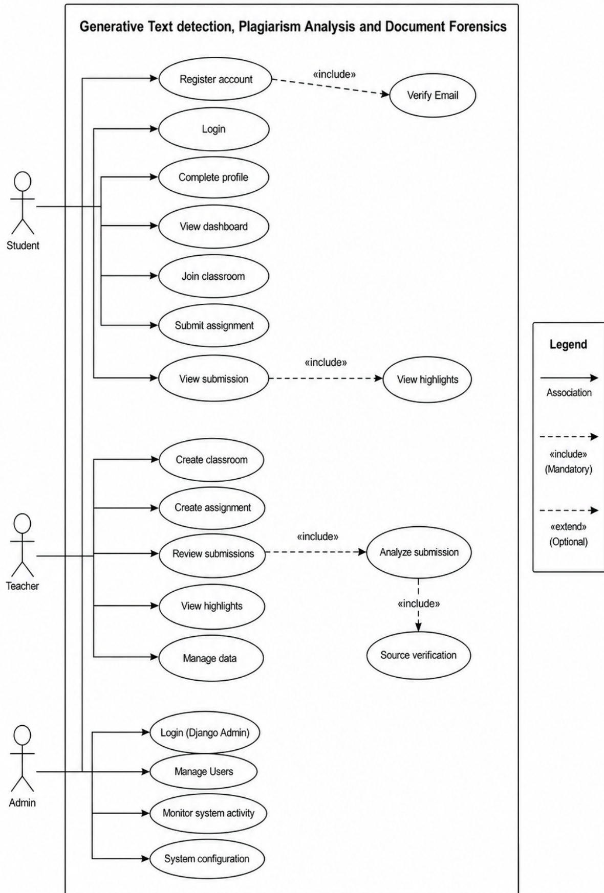
Figure 1: Use Case Diagram of the System
