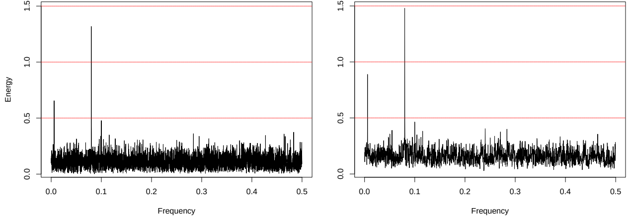
Figure 8: Spectral density (energy) based on FFT (left) and on KZFT_{\nu,4201,6} to produce the KZ-periodogram (right)
