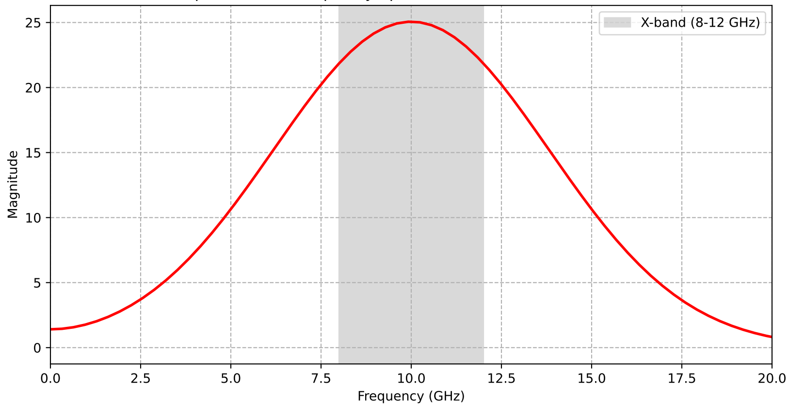
Requirement 4: Frequency Spectrum (FFT) of the Source Pulse
