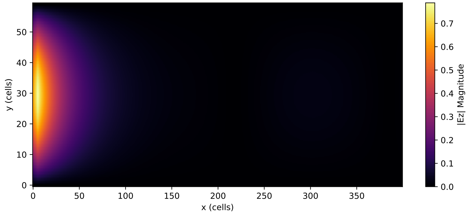
Plot 2: 2D Snapshot (7.0 GHz)
