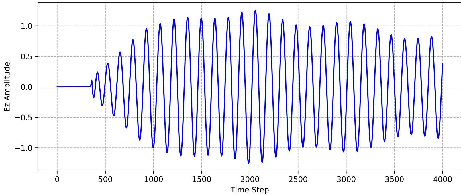
Plot 3: Time-Domain Signal at Probe (11.0 GHz)
