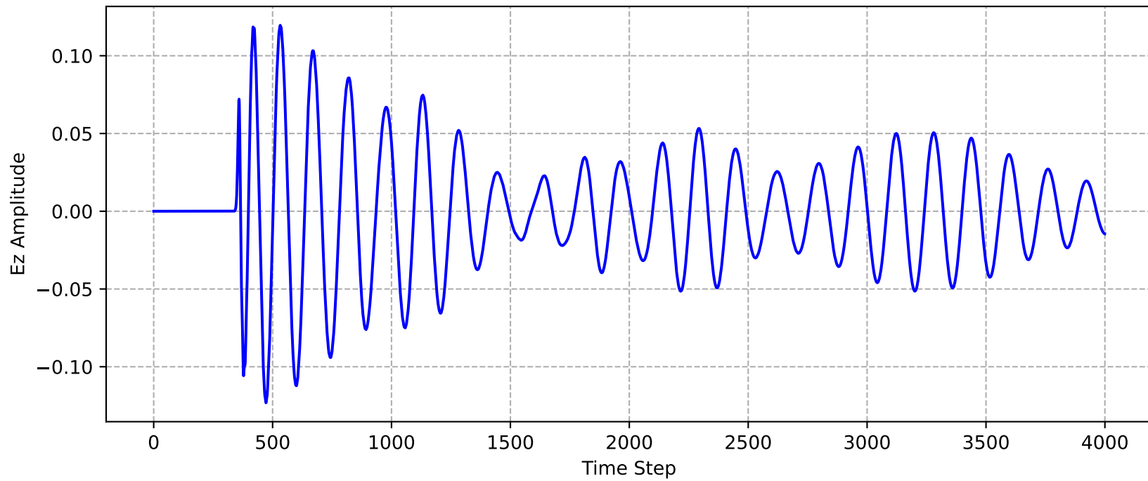
Plot 3: Time-Domain Signal at Probe (7.0 GHz)
