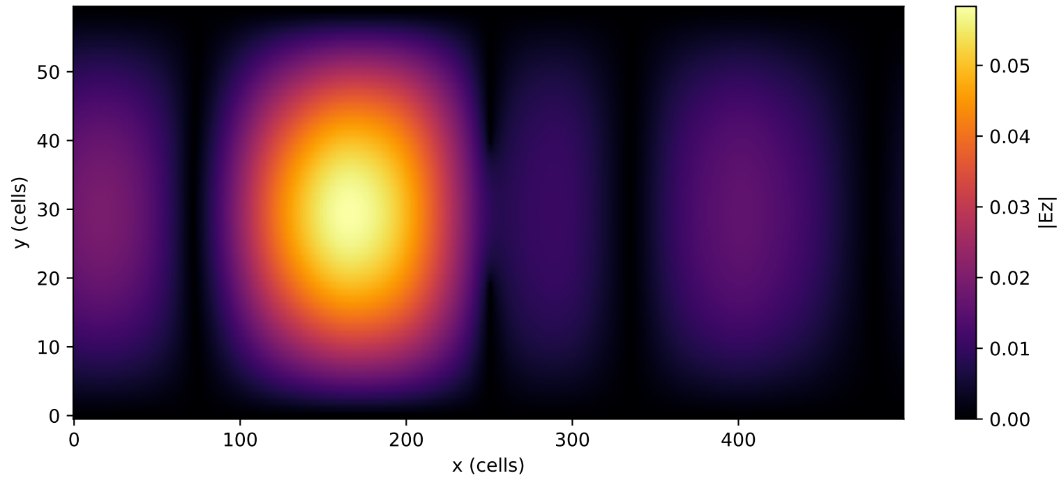
2D E field: Diffraction
