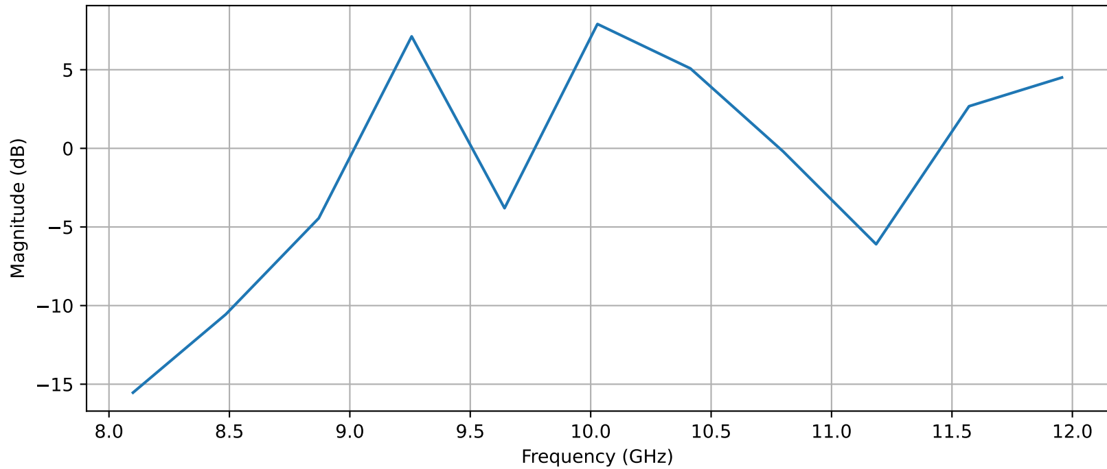
|S11| Return Loss
