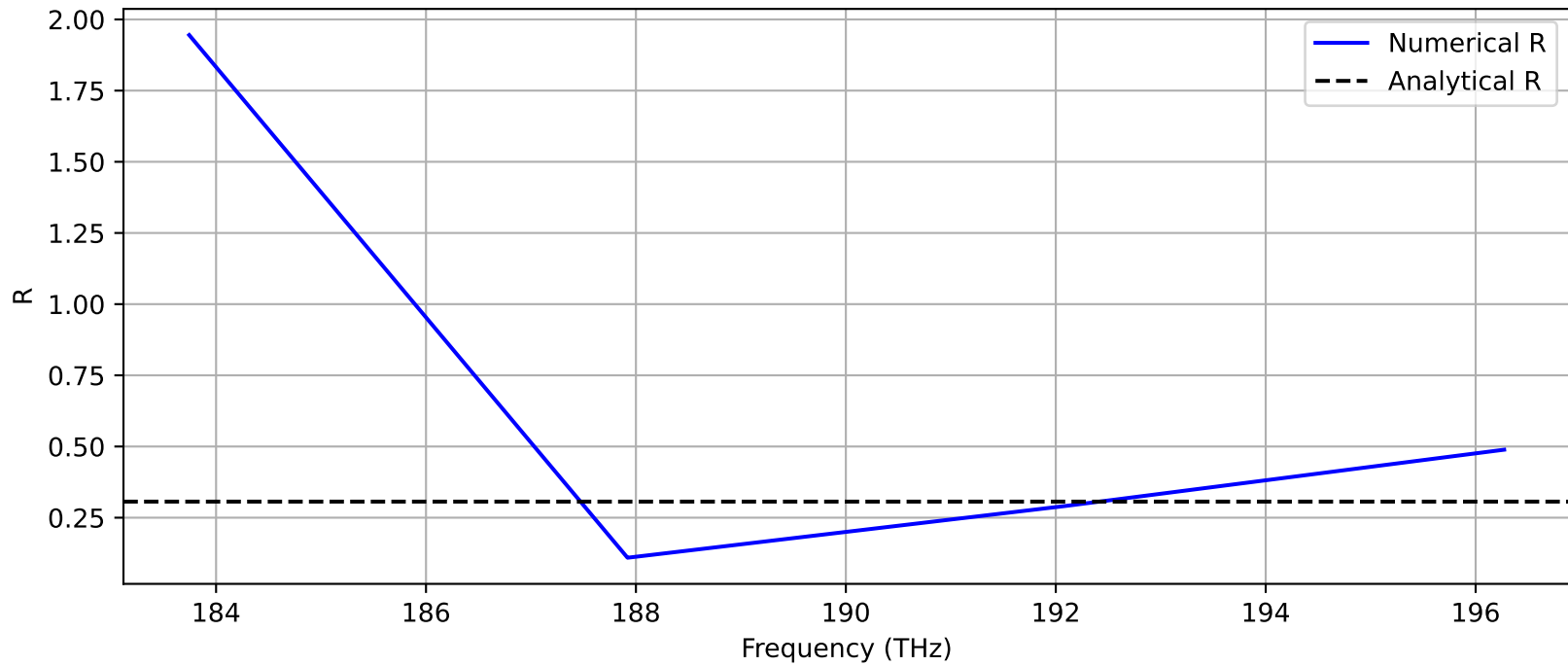
3. Reflection Coefficient (R) vs Frequency
