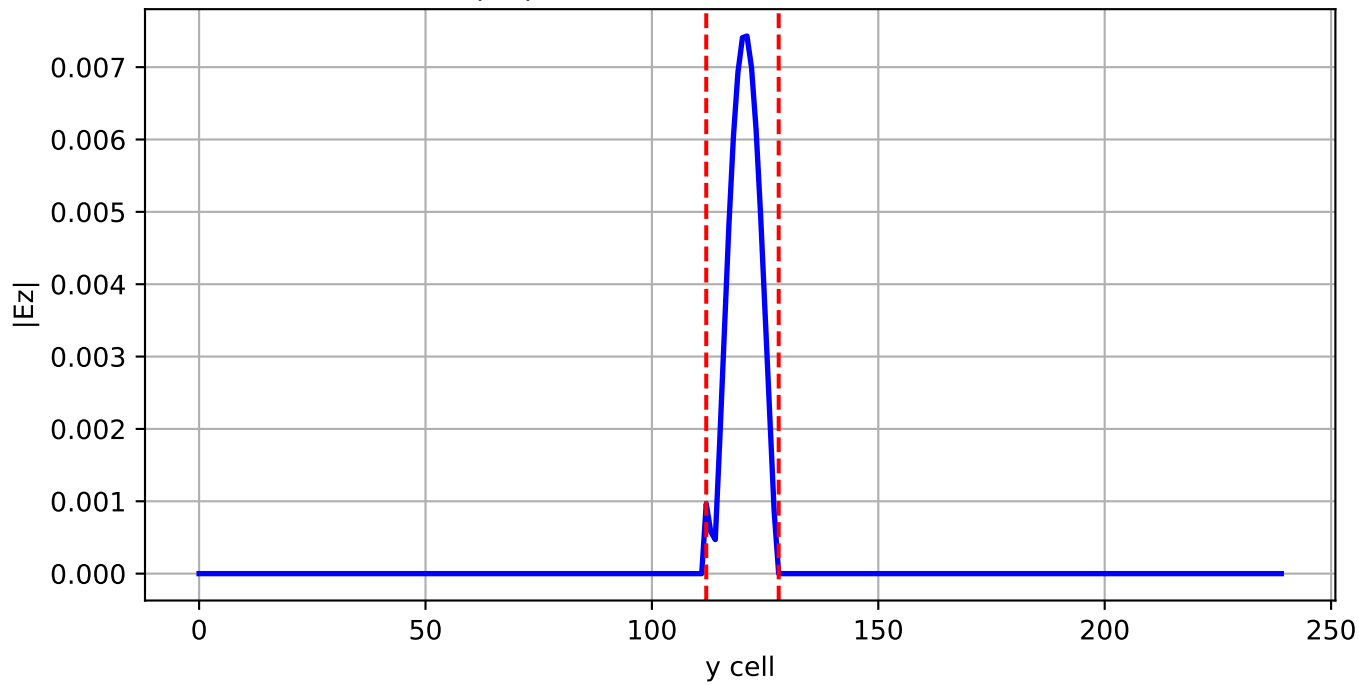
2. |E_z| Sampled Across Aperture Plane
