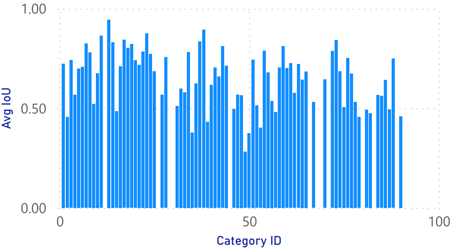
Avg IoU by category_id
