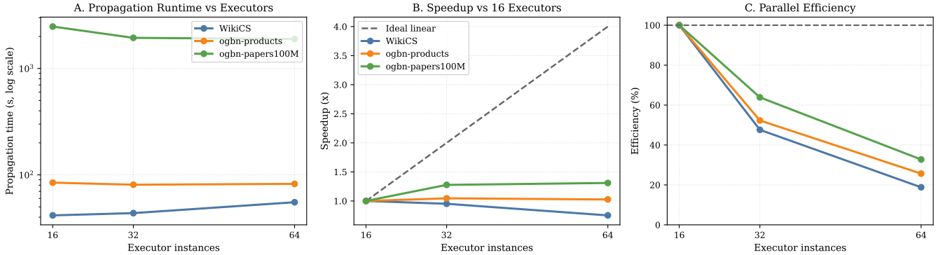
Figure 3. Phase 3.7/3.8 executor-scaling behavior across three graph sizes for two-hop propagated features [x^{(0)} || x^{(1)} || x^{(2)}] . Panel A shows propagation runtime on a log scale. Panel B compares observed speedup to ideal linear scaling from 16 executors. Panel C reports parallel efficiency, highlighting diminishing returns at higher executor counts.
