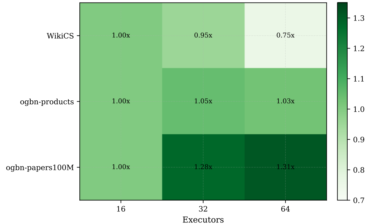
B. Speedup vs 16 Executors
