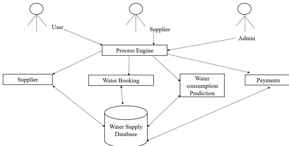
Figure 4.1: System Architecture
