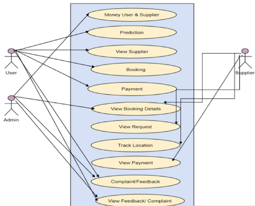
Figure 6.2: Usecase Diagram
