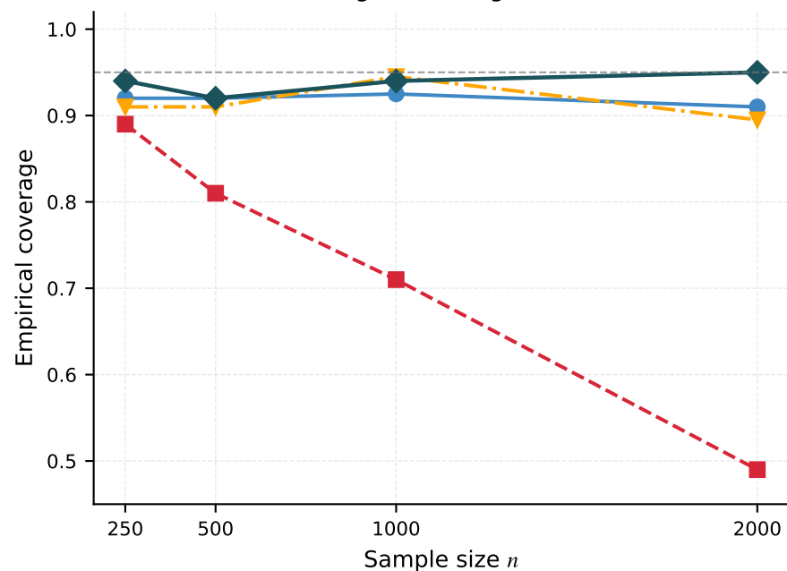
Scaling of coverage with n
