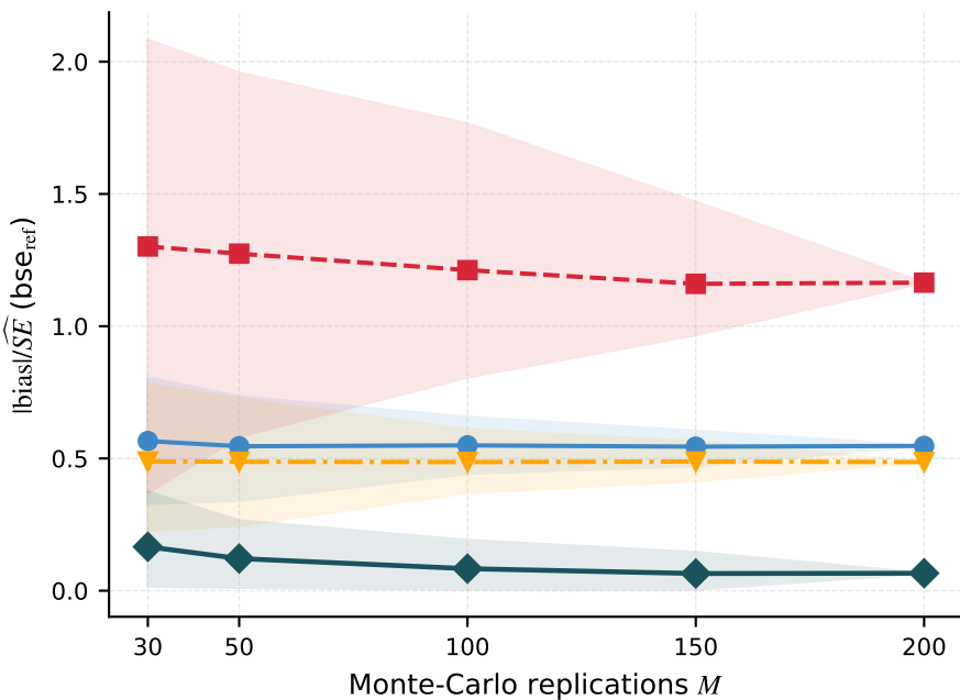
Stabilisation of bse with M
