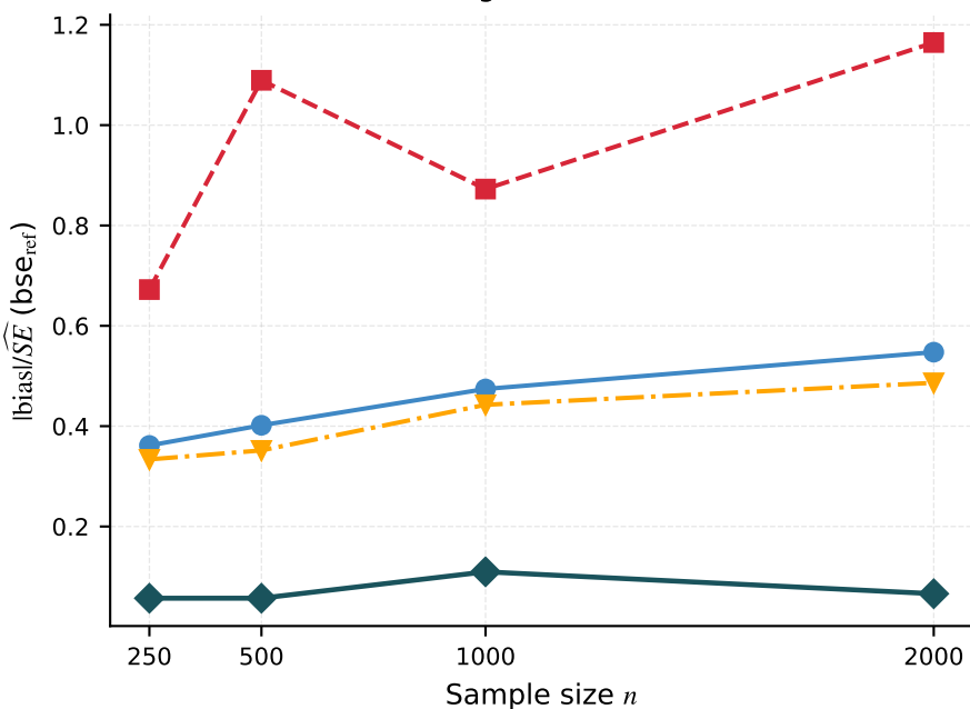
Scaling of bse with n
