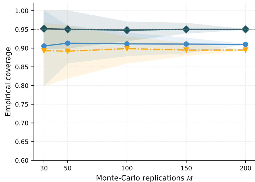
Stabilisation of coverage with M
