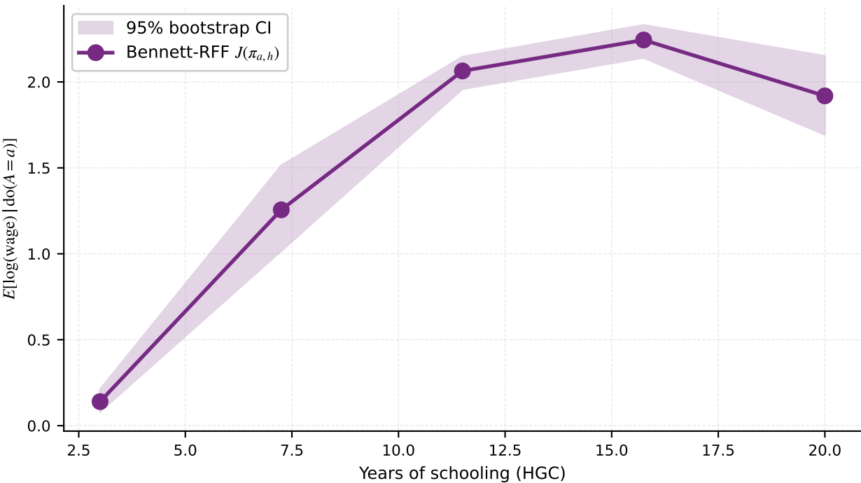
Bennett dose-response — NLSY79 — return to schooling
