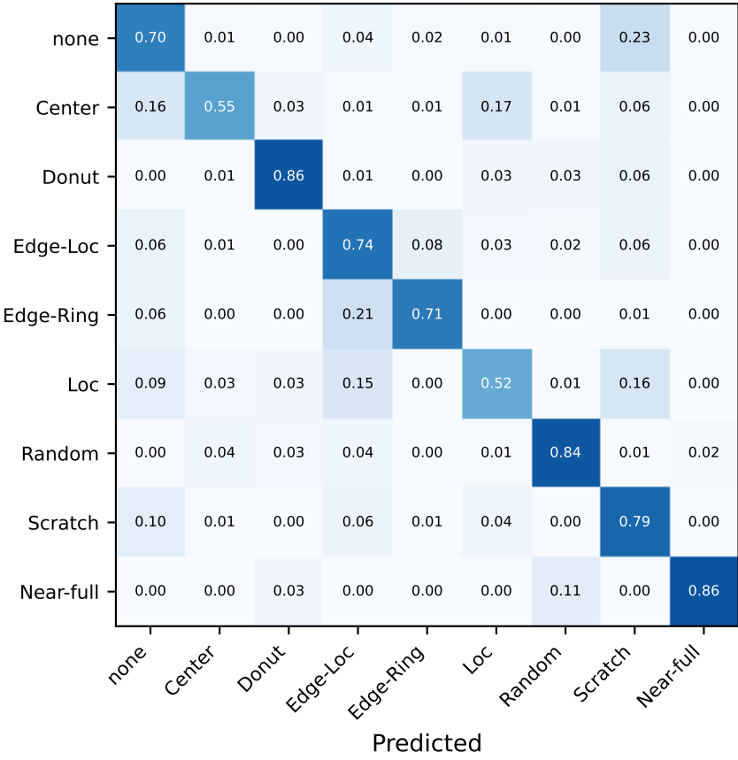
E2CNN, balancing (cost matrix)
