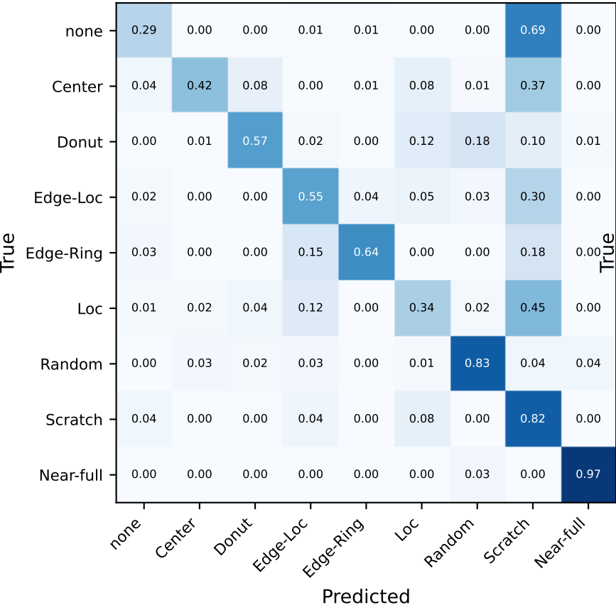
CNN, balancing (cost matrix)
