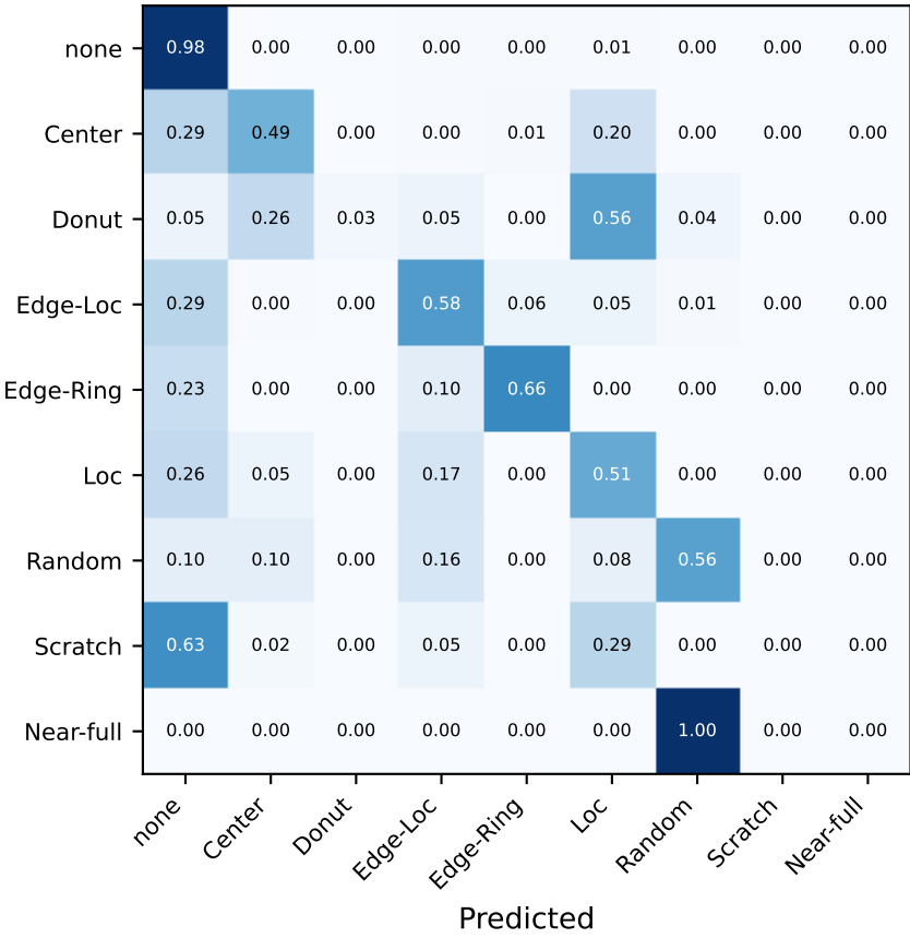
CNN, no balancing (cost matrix)
