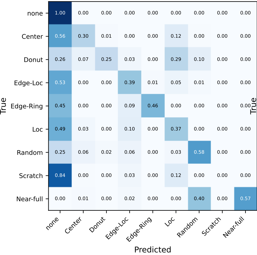
Plain CNN
