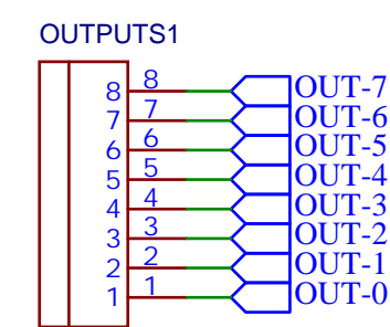
Outputs to relays modules
