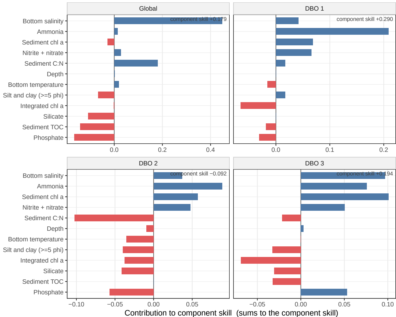
Dynamic model, total biomass, train/test: SHAP attribution
