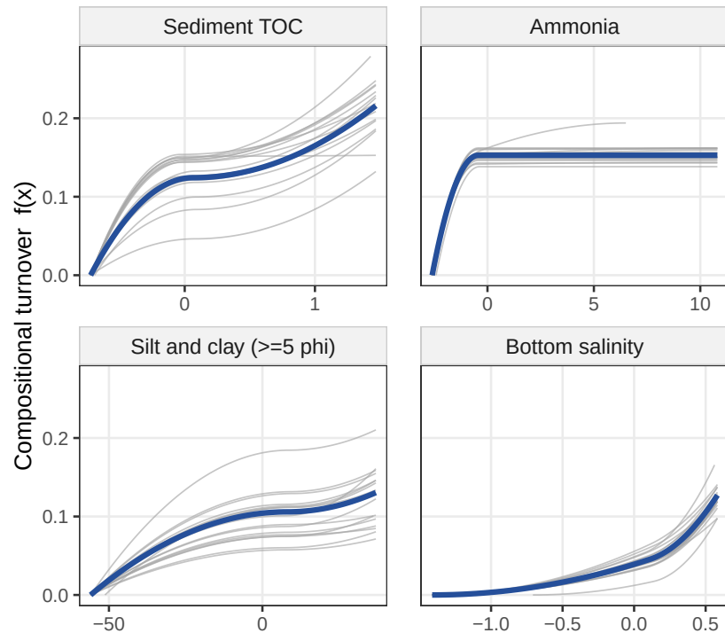
b Fitted relationships, 4 strongest environmental variables
