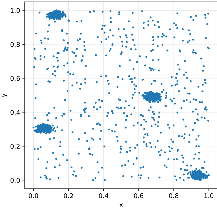
Noisy blobs
