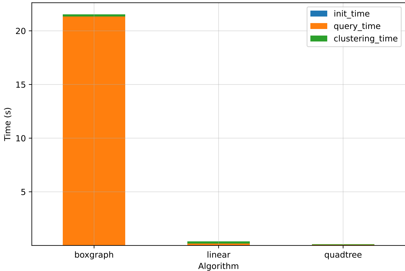
Runtime Breakdown
