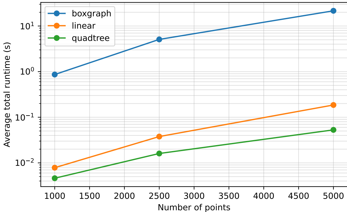
Runtime vs Number of Points
