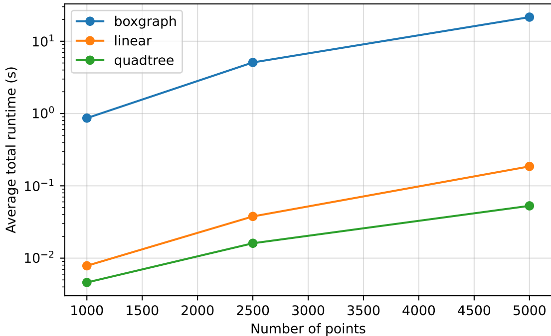
Runtime vs n (clean_blobs)
