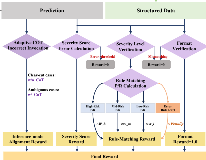
(b) Refining Severity-Aware Ranking with RL
