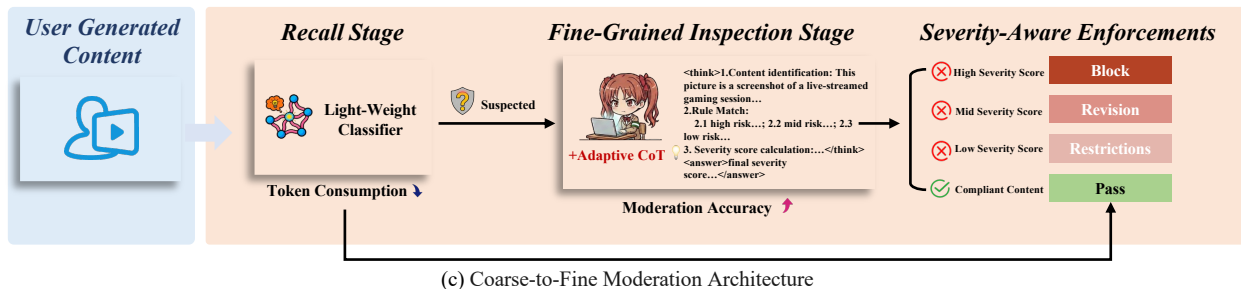
(c) Coarse-to-Fine Moderation Architecture
