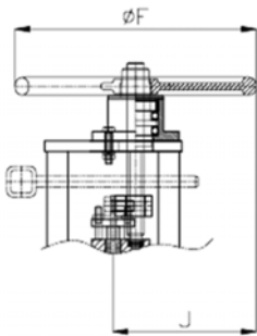
1) 2~4" Hand Wheel
