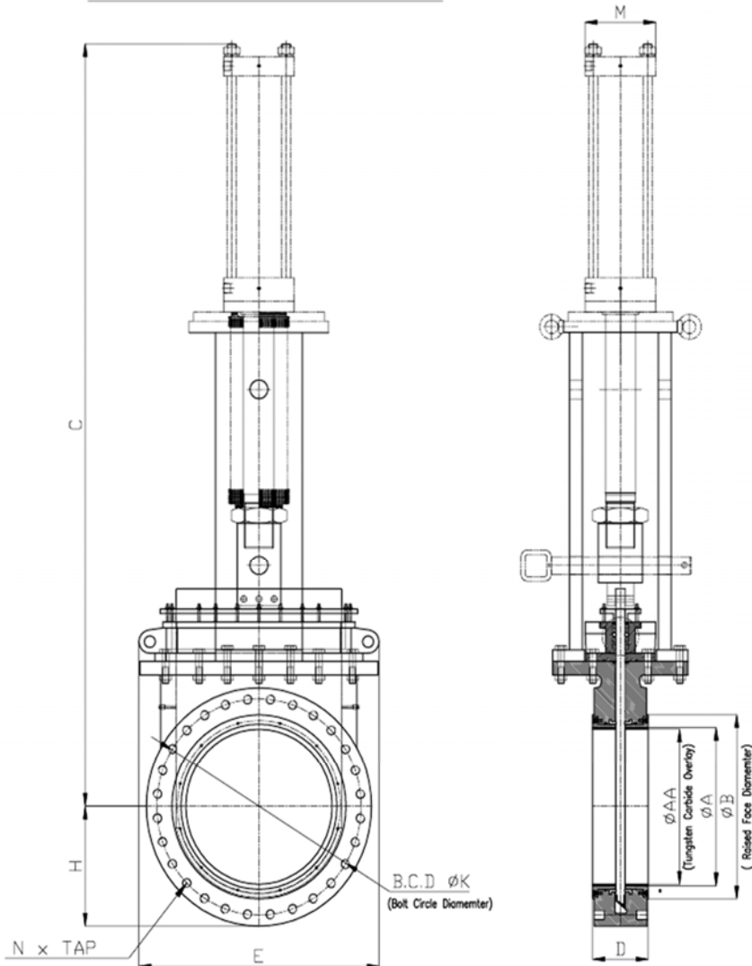
3) 12~60" Hydraulic Cylinder
