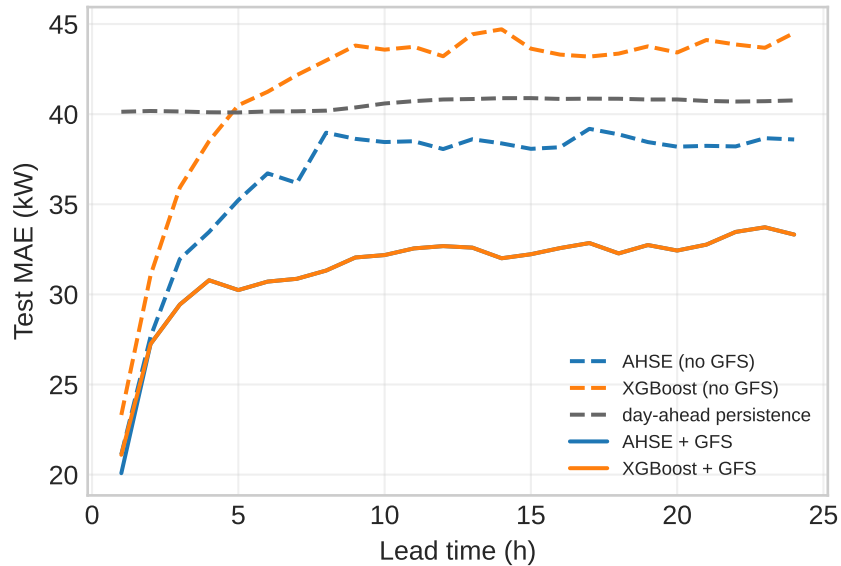
Yulara (uncurtailed sites, 768 kW)
