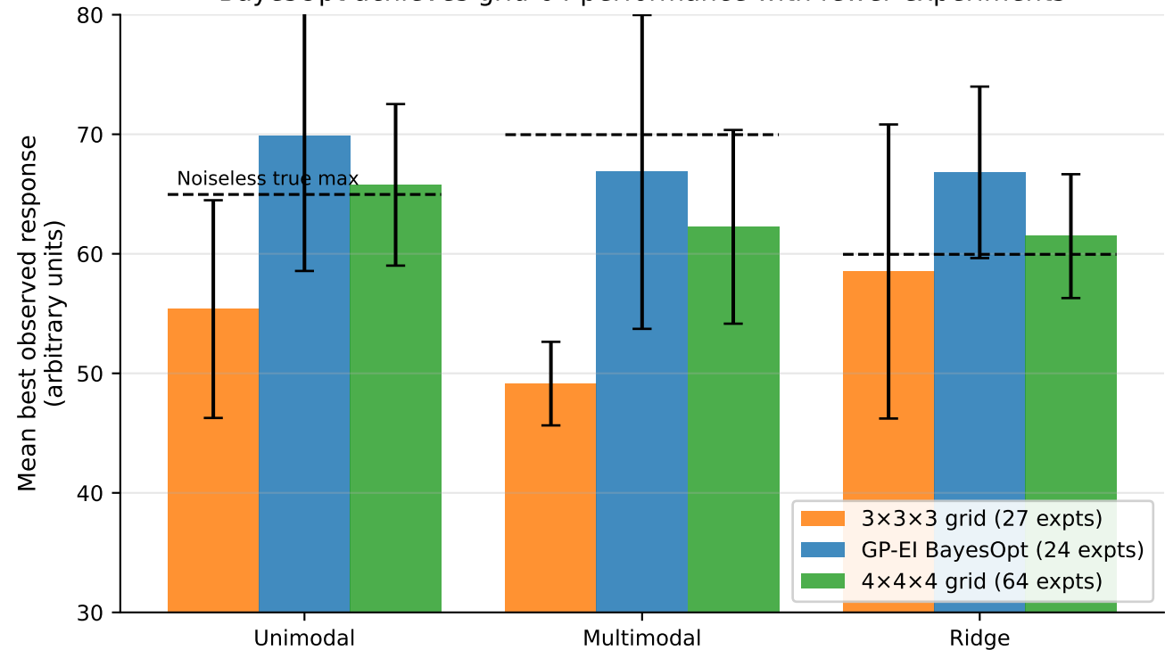
BayesOpt achieves grid-64 performance with fewer experiments
