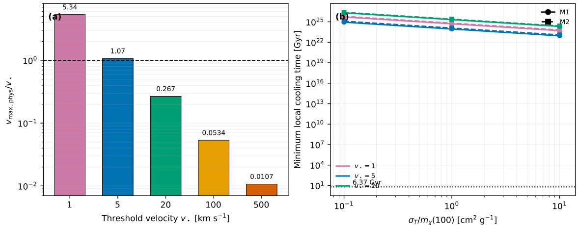
Figure 3: Physical activity audit. (a) Maximum physical one-dimensional dispersion divided by the emission threshold; the dashed line marks unity. (b) Minimum exact local cooling time for the finite-kernel branches. Colors denote thresholds and line styles denote emission channels. The dotted line marks the 6.37 Gyr cosmic age at the lens redshift.
