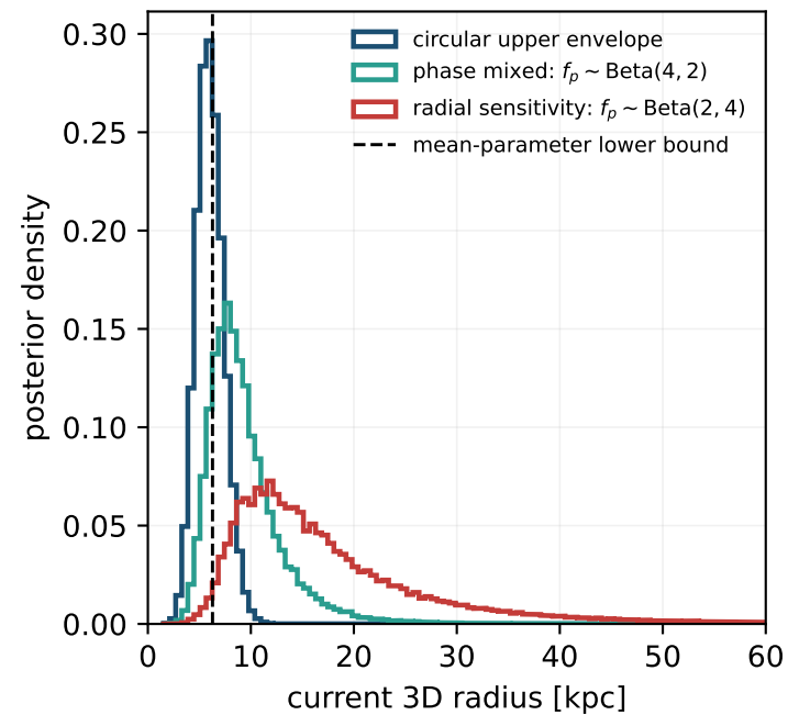
(a) deprojected location
