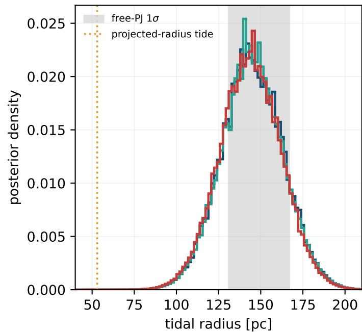
(c) imaging-conditioned tide
