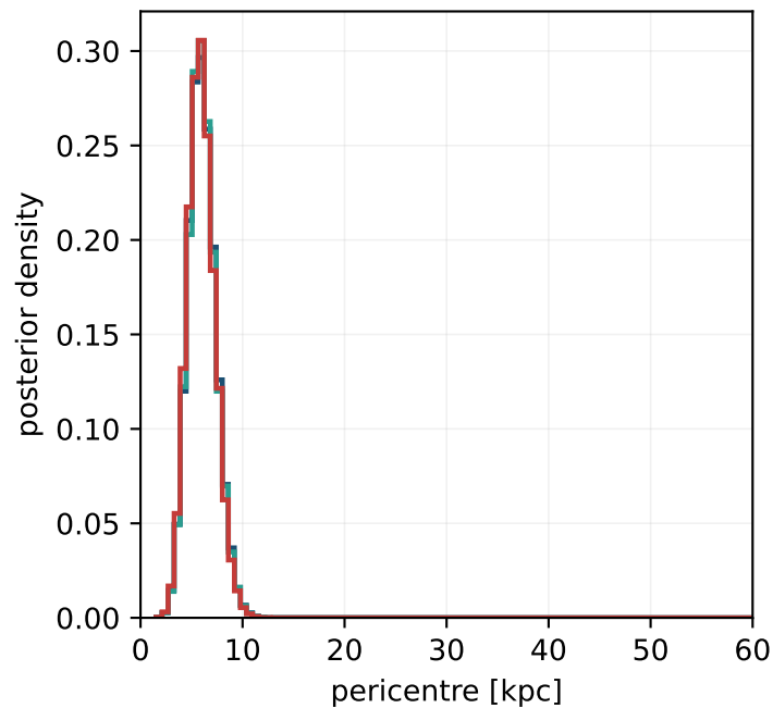
(b) tidal-setting orbit
