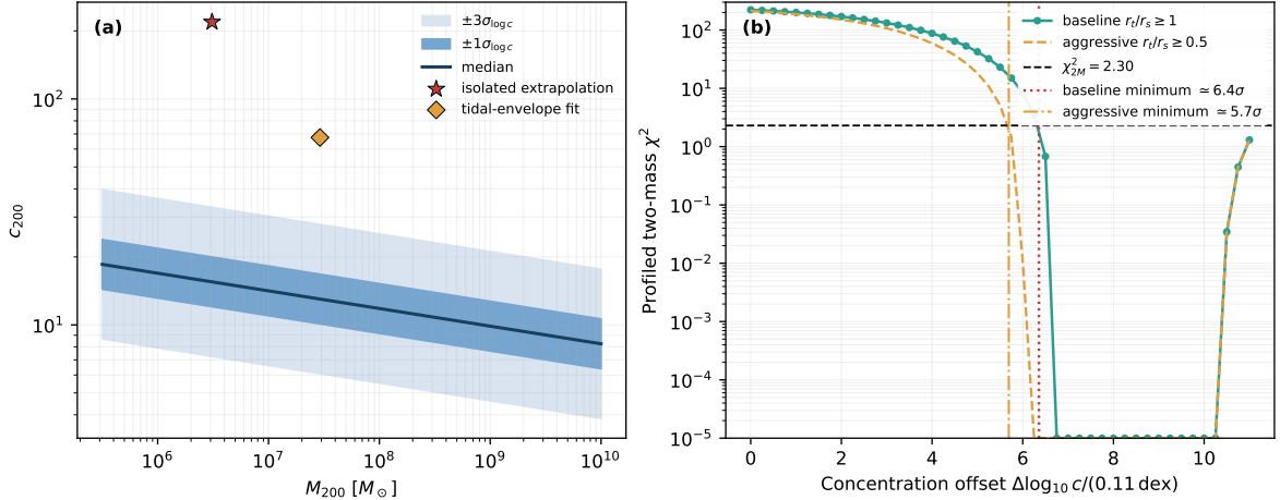
Figure 5: Cosmological and tidal-envelope plausibility audit. (a) The Dutton & Macciò (2014) median concentration relation at z = 0.881 , with one- and three-sigma bands, compared with the isolated extrapolation and the first baseline tidal-envelope grid point inside the reference contour. (b) Two-mass \chi^2 profiled over M_{200} and BMO truncation at fixed concentration offset. The baseline has r_t/r_s \geq 1 ; the aggressive sensitivity branch extends to 0.5. Offset labels are in units of the assumed 0.11-dex scatter and are not formal statistical significances.
