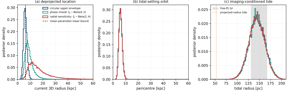
Figure 6: Host-orbit and tidal sensitivity audit conditioned on the published free pseudo-Jaffe summaries. (a) Current three-dimensional radius for the circular upper envelope, phase-mixed prior, and radially biased sensitivity prior. The dashed line is the lower bound evaluated at the mean measured mass and truncation radius; measurement uncertainty permits posterior samples below it. (b) Pericenter distributions that set the tidal radius. (c) Imaging-conditioned tidal-radius distributions; the gray band is the published free-PJ 1\sigma interval and the dotted line is the tidal radius obtained by setting the three-dimensional radius equal to the projected one. The curves use one-dimensional public summaries rather than the unavailable correlated PRONTO samples and are not formal orbit constraints.
