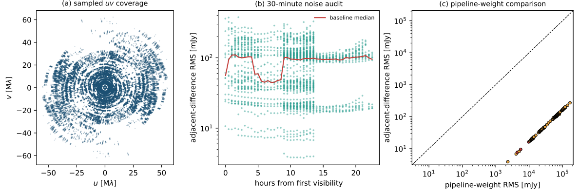
Figure 7: Public GM068 UVFITS quality audit: sampled uv coverage, 30-minute adjacent-difference noise estimates, and a baseline-level comparison with the pipeline-weight RMS. The public AIPS weights and amplitudes have an arbitrary overall normalization, so the figure supports reproducibility of selection and internal noise weighting, not an absolute flux-calibration claim.
