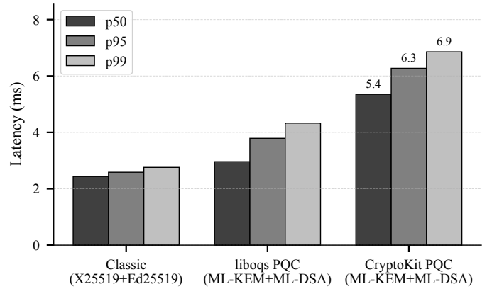
Fig. 8. Handshake latency percentiles for Classic, liboqs PQC, and CryptoKit PQC (warmup=10; N=1000 for Classic/liboqs, N=5000 for CryptoKit). Data source: handshake_bench_2026-01-23.csv. Values align with Table 18 and Supplementary Table S1.
