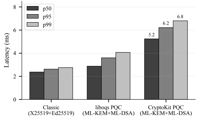
Fig. 8. Handshake latency percentiles for Classic, liboqs PQC, and CryptoKit PQC (warmup=10; N=1000 for Classic/liboqs, N=5000 for CryptoKit). Data source: handshake_bench_2026-01-23.csv. Values align with Table 10 and Supplementary Table S12.
