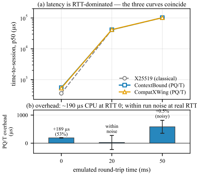
Fig. 6. Time-to-session under real to netem (mean of two repetitions). (a) latency is RTT-dominated—the three curves coincide. (b) the overhead is \sim 190 \mu s of CPU at RTT 0; at realistic RTT it is within run-to-run noise (error bars span the two repetitions and cross zero at RTT 20 ms).
