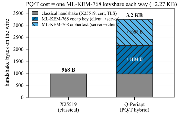
Fig. 7. TLS 1.3 key-exchange wire-budget increment only. The PQ/T cost is one ML-KEM-768 keyshare each way (+2.27 KB) on top of the classical group; it excludes the authentication certificate/signature bytes, which are unchanged from the classical baseline in the rustls measurement. (The ML-DSA-authenticated demo’s multi-KB signature is a separate budget, not shown here.)
