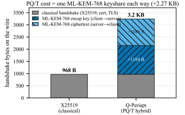
Fig. 7. TLS 1.3 key-exchange wire-budget increment only. The PQ/T cost is one ML-KEM-768 keyshare each way (+2.27 KB) on top of the classical group; it excludes the authentication certificate/signature bytes, which are unchanged from the classical baseline in the rustls measurement. (The ML-DSA-authenticated demo’s multi-KB signature is a separate budget, not shown here.)
