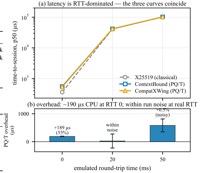
Fig. 5. Time-to-session under real tc netem (mean of two repetitions). (a) latency is RTT-dominated—the three curves coincide. (b) the overhead is \sim 190 \mu s of CPU at RTT 0; at realistic RTT it is within run-to-run noise (error bars span the two repetitions and cross zero at RTT 20 ms).
