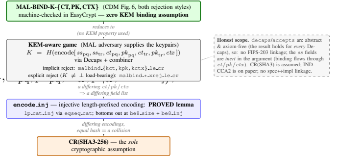
Fig. 2. The kernel as a reduction tower: MAL-BIND-K- \{\text{CT}, \text{PK}, \text{CTX}\} (CDM Figure 6, both rejection styles) reduces—using no property of Decaps—through the proved encode_inj to collision-resistance of SHA3, the sole cryptographic assumption.
