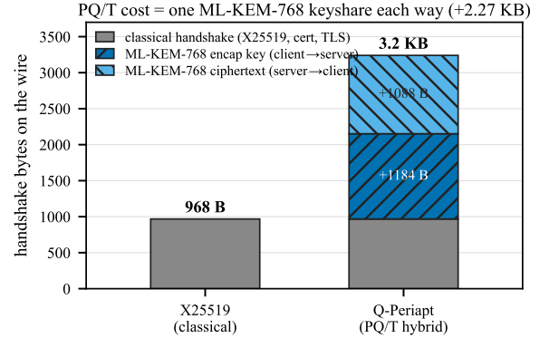
Fig. 6. Handshake wire budget. The PQ/T cost is one ML-KEM-768 keyshare each way ( +2.27\text{ KB} ), which fits inside the existing flights.
