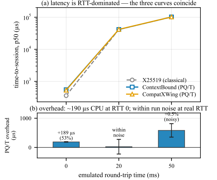
Fig. 5. Time-to-session under real tc netem (mean of two repetitions). (a) latency is RTT-dominated—the three curves coincide. (b) the overhead is \sim 190\mu\text{s} of CPU at RTT 0; at realistic RTT it is within run-to-run noise (error bars span the two repetitions and cross zero at RTT 20 ms).
