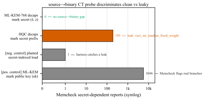
Fig. 4. The source \rightarrow binary CT probe discriminates: the genuine ML-KEM secret yields zero flags; the same harness flags HQC’s constant-weight sampler (193) and validates itself with two controls.
