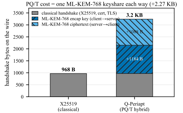
Fig. 7. Handshake wire budget. The PQ/T cost is one ML-KEM-768 keyshare each way (+2.27 KB), which fits inside the existing flights.
